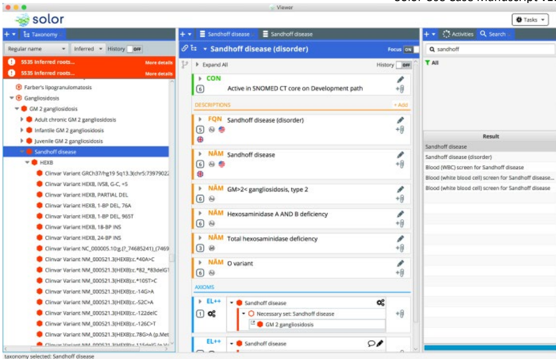
Figure 2: Solor GUI
