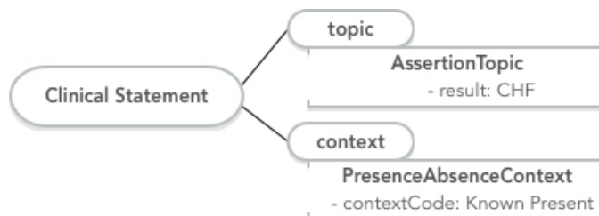
Figure 9.3. Patient has diagnosis of congestive heart failure.
