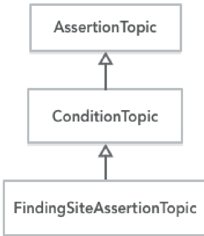
Figure 9.8. Assertion Hierarchy
