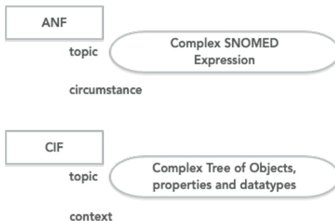
Figure 9.14. Topic Comparison
