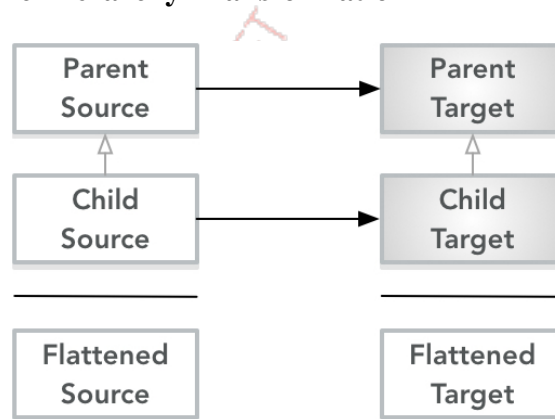
Figure 7.7. Symmetric Hierarchy Transformation
