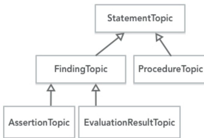
Figure 9.5. Topic Hierarchy
