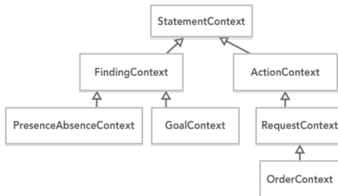
Figure 9.11. Procedure Hierarchy
