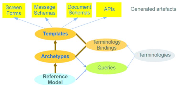
Figure 6.3. OpenEHR architecture
