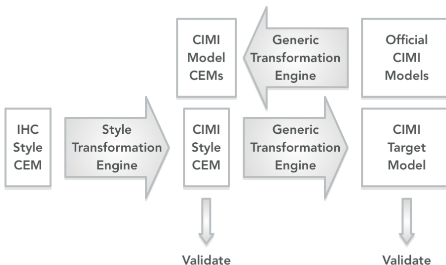
Figure 7.8. Transformation Strategy
