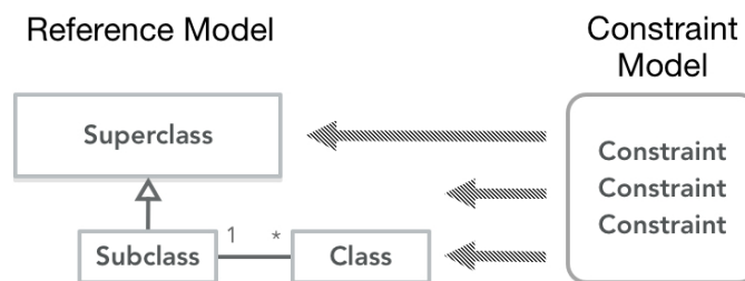
Figure 7.1. Reference Model Constraint Paradigm
