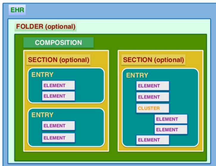
Figure 6.4. OpenEHR Reference Model
