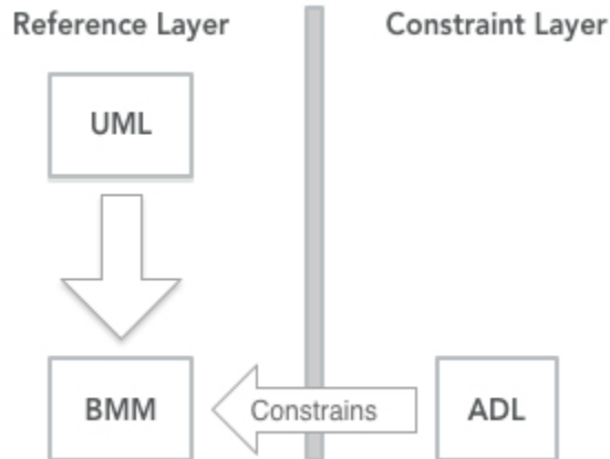
Figure 9.1. CIMI CIF Model Layers
