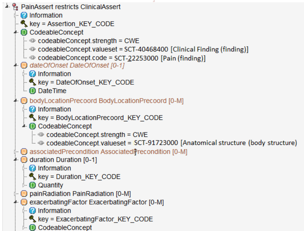
Figure 10.8. An alternative CIMI DCM for pain observations.
