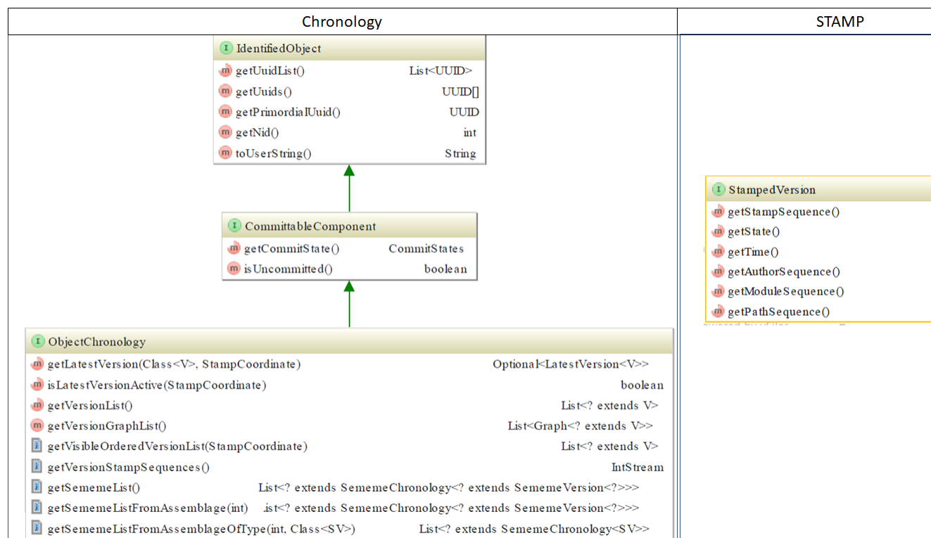
Figure 2.2. Chronology and STAMP
