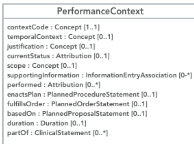
Figure 15.12. PerformanceContext
